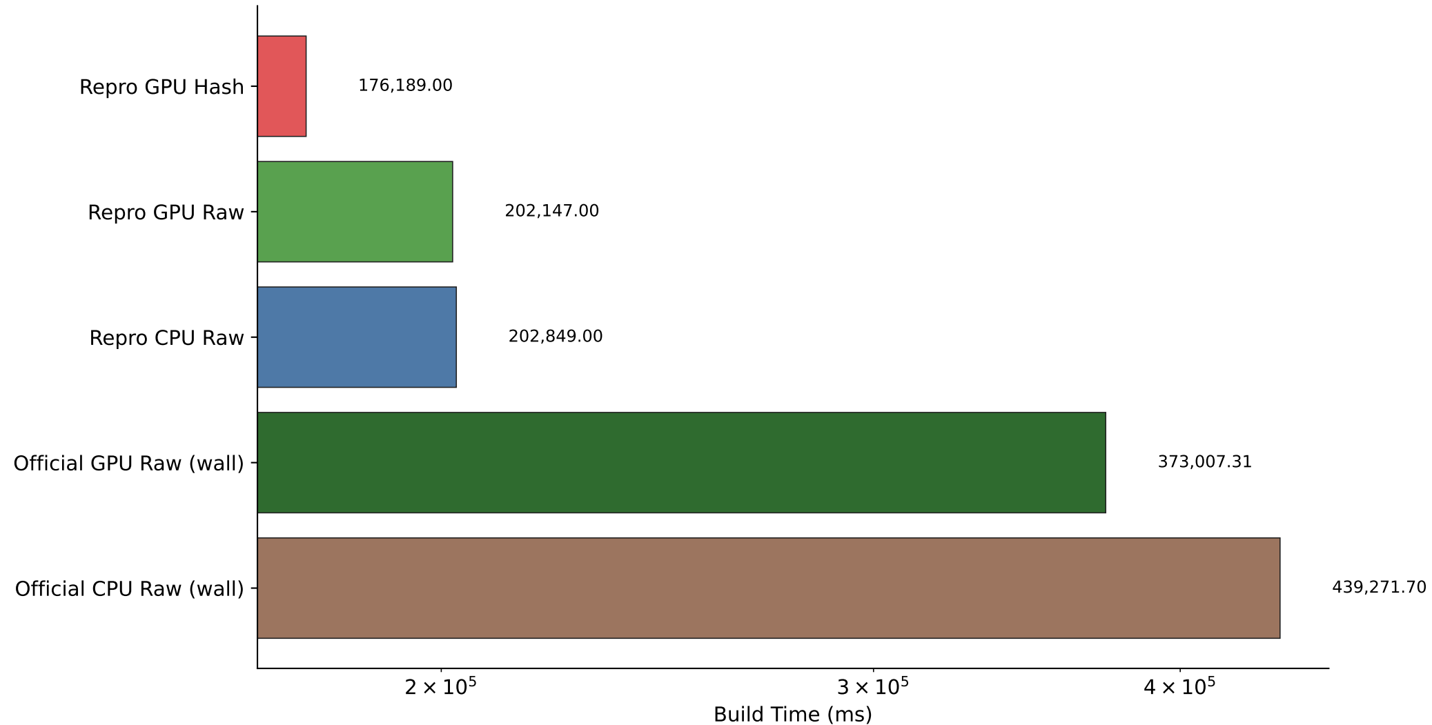
Detailed Build Time (ms) Comparison
