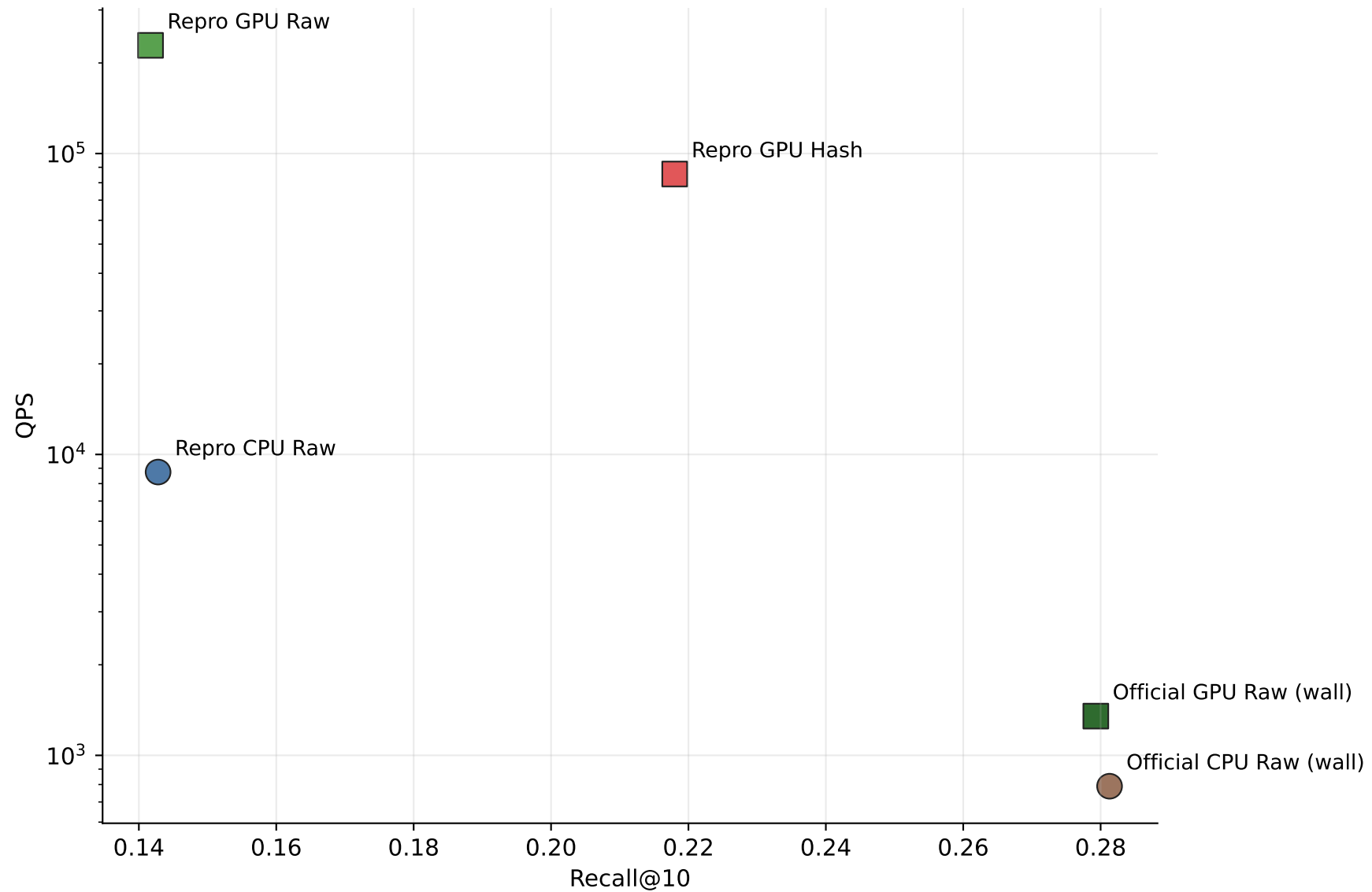
Recall / QPS trade-off
