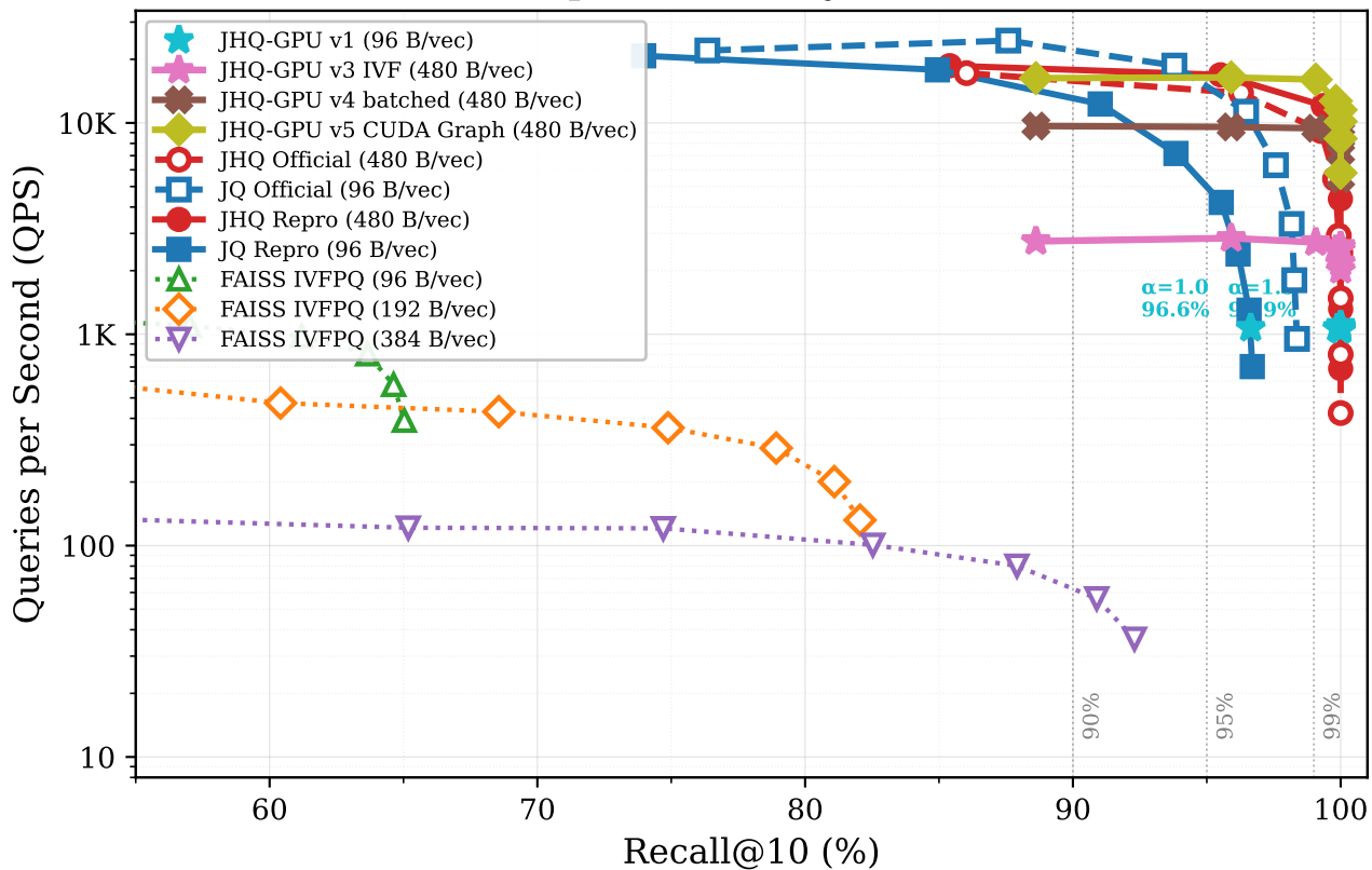
(a) Speed-Accuracy Trade-off
