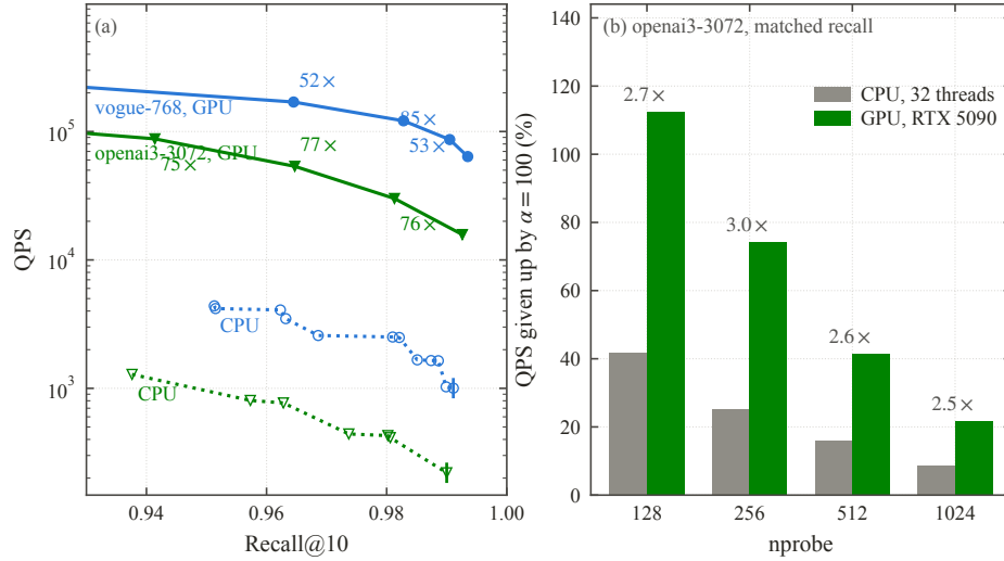
Fig. 4: GPU against CPU JHQ at the same index parameters. (a) Both sides’ ( \alpha , nprobe ) envelopes, annotated with the ratio at matched recall; open markers are the CPU points the envelope is taken over. (b) What the \alpha budget is worth on each processor, at matched recall on openai3-3072 — the reason the budget is worth choosing on a GPU and not on a CPU.
