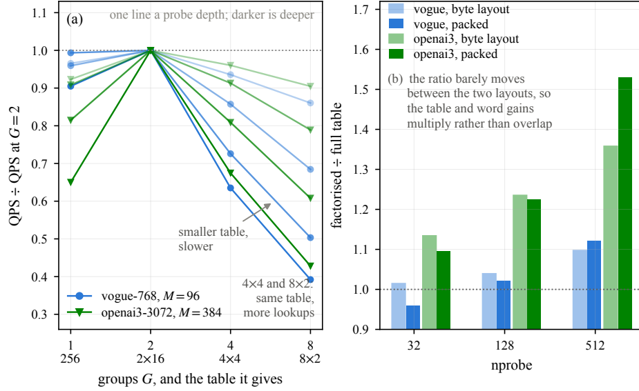
Fig. 7: Why the exact LUT is split into two groups. (a) G=2 is never beaten, although G=4 and G=8 use smaller tables and are byte-identical to each other, exposing the lookup-instruction trade-off; (b) factorisation matters far more at M=384 than M=96 and remains complementary to packed loading. Panel (b) is the two-by-two layout phase, measured at nprobe \in \{32, 128, 512\} ; the nprobe=8 point quoted in the text is the lightest probe-depth line of panel (a).
