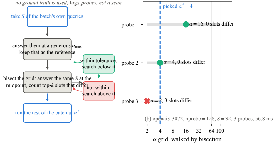
Fig. 4: Label-free output-stability calibration. Ground truth is not used during \alpha selection.
