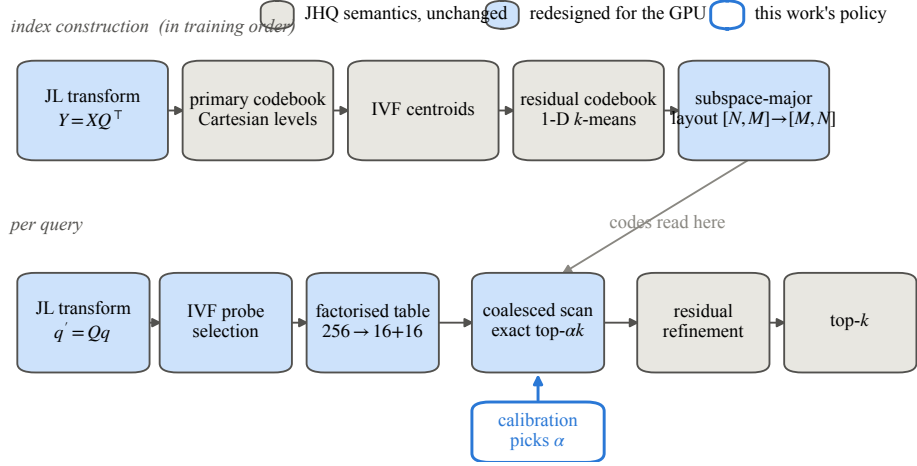
Fig. 1: JHQ build and query pipeline. GPU redesign changes execution and physical layout while preserving the original hierarchy. The scan uses bounded per-thread top- \alpha k selection; Proposition 1 characterises the ideal exact selector, while Section 4.3 quantifies the implementation’s measured deviation.
