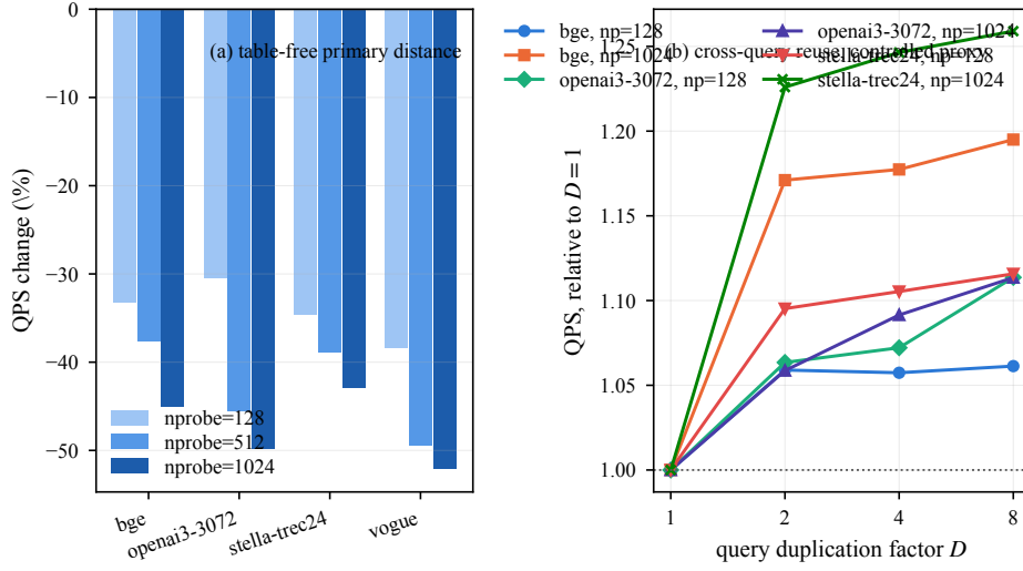
Fig. 8: Negative controls for mechanism. (a) Table-free exact primary distance reduces LUT state yet loses 30–52%; (b) controlled query duplication isolates cross-query reuse and shows only modest additional throughput. These reject simplistic “fewer bytes is always faster” and “reuse alone will solve the scan” explanations.
