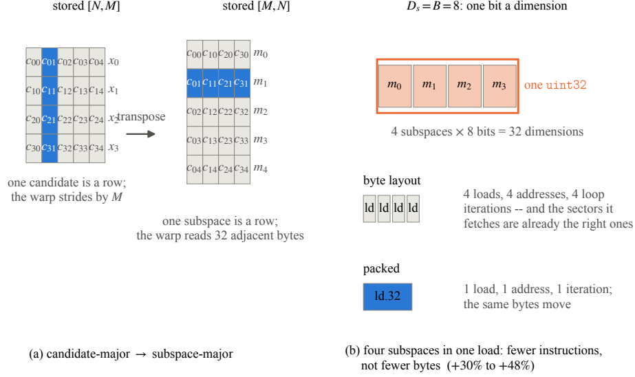
Fig. 2: Logical candidate-major versus GPU scan layout, and the separate role of packed 32-bit access.
