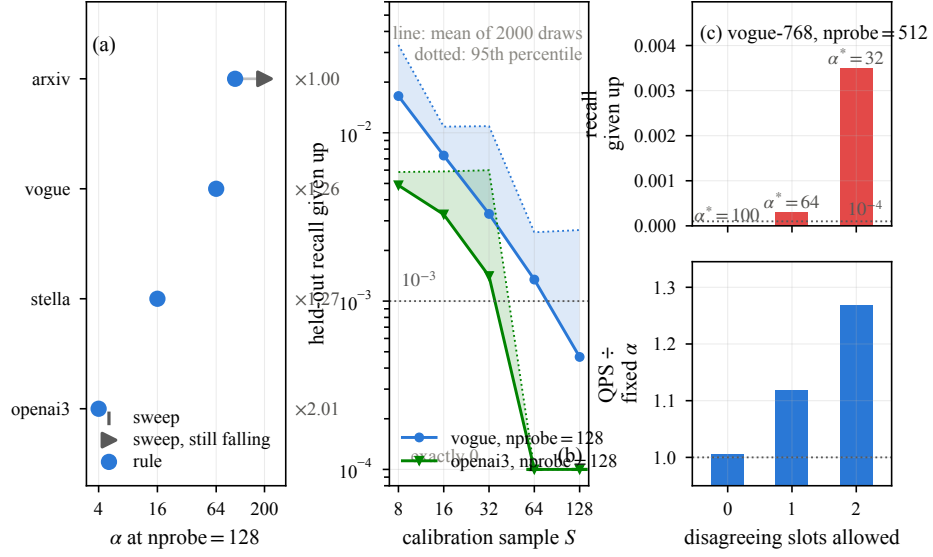
Fig. 6: Calibration validation. (a) Selected \alpha versus the exhaustive sweep where a same-operating-point sweep exists, annotated with the throughput the selection gains; (b) held-out resampling shows that sample-size risk is workload dependent; (c) tolerance changes the selected budget and quality–cost trade-off.
