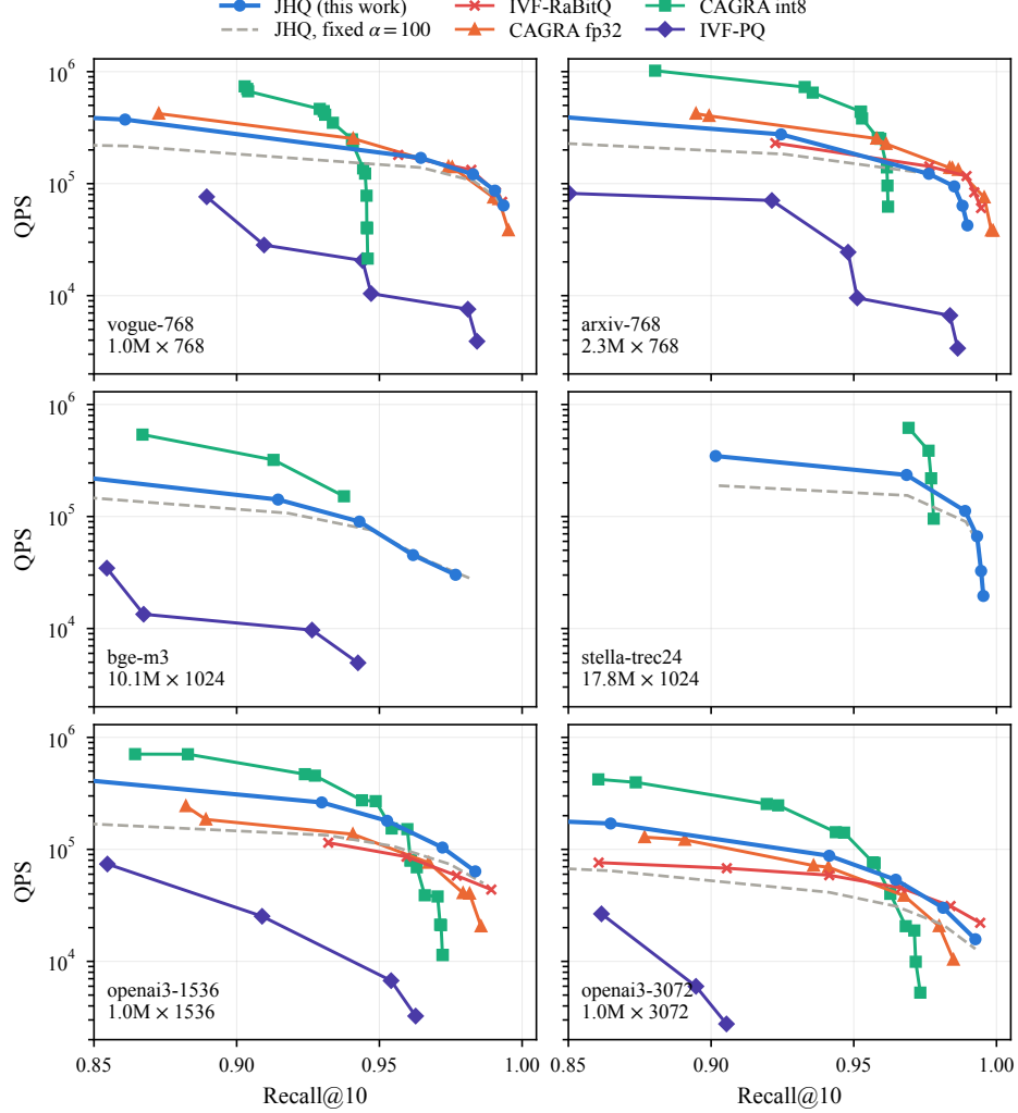
Fig. 5: Measured Recall@10–QPS frontiers across all six datasets, at batch 1,024. Four datasets include complete JHQ/IVF-RaBitQ curves; the two larger datasets show the baselines available on the tested GPU. Sweep endpoints are measured endpoints, not architectural recall ceilings.
