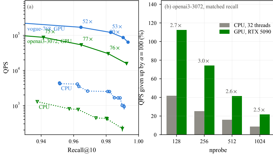
Fig. 10: CPU baseline. (a) Both devices’ ( \alpha , nprobe ) envelopes, with the matched-recall ratio annotated only where both cover the recall; the tick marks where the CPU envelope ends. (b) The cost of pinning \alpha=100 at matched recall is 2.5–3 \times larger on the GPU than on the CPU at every probe depth.
