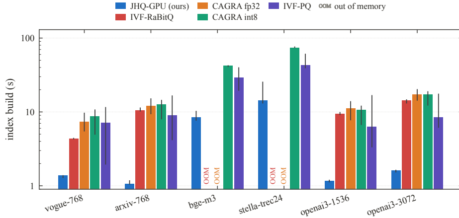
Fig. 4: Index build time, log scale. Bars are the median over swept configurations and repeat builds and whiskers their range, not a confidence interval. JHQ’s bar is one cold training plus its median encode: training is cached after a dataset’s first row and encoding is not. Each baseline’s fastest build per dataset is used. The coarse-training budgets differ and are not controlled here: JHQ trains at 39 points a centroid, cuVS defaults to 256, so IVF-RaBitQ trains on 5.8 to 6.6\times as many points. Part of its build gap is that budget rather than the index, and the same budget buys it better centroids at search time.
