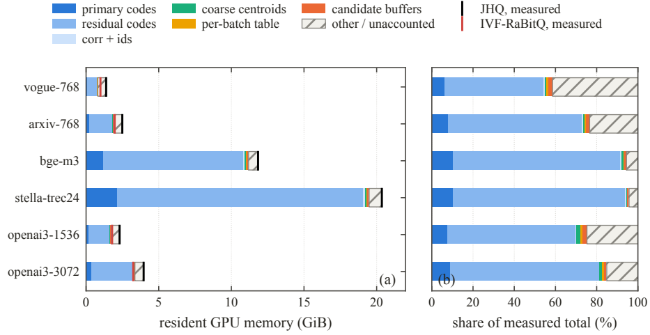
Fig. 8: Where the resident index sits, by component. (a) Absolute, with the measured totals for JHQ and IVF-RaBitQ marked; (b) the same as shares. The hatched band is measured total minus the components we can attribute, and is shown rather than folded into one of them.
