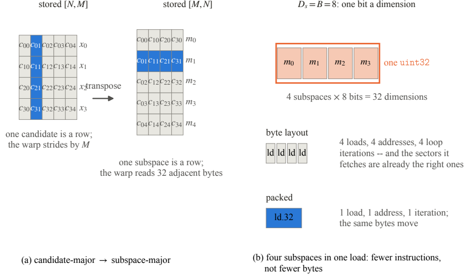
Fig. 1: Two rearrangements of the same bytes, neither of which changes a distance. (a) Storing the primary codes subspace-major rather than candidate-major turns a warp’s strided read into 32 adjacent bytes. (b) At D_s=B=8 four subspaces are 32 dimensions and fit one uint32 , so four loads, four addresses and four loop iterations become one. Section 6.4 measures what that is worth.
