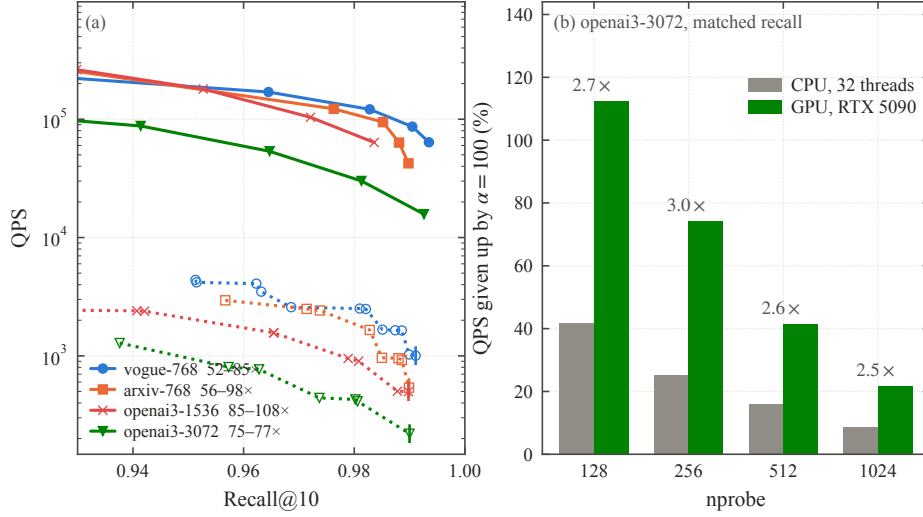
Fig. 7: GPU against CPU JHQ at the same index parameters, on the four datasets the CPU reference covers. (a) Both sides’ ( \alpha , nprobe ) envelopes: solid is the GPU, dotted with open markers the CPU points the envelope is taken over, and the legend gives each dataset’s range of matched-recall ratios. (b) What the \alpha budget is worth on each processor, at matched recall on openai3-3072 — the reason the budget is worth choosing on a GPU and not on a CPU.
