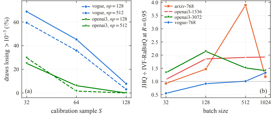
Fig. 6: Sensitivity to the two knobs the evaluation varies. (a) The share of 64 random calibration samples that give up more than 10^{-3} of held-out recall, against the sample size S ; solid is np=128 , dashed 512. (b) JHQ over IVF-RaBitQ at matched Recall@10 of 0.95, against batch size, on the four datasets IVF-RaBitQ builds on; above 1 is JHQ ahead.
