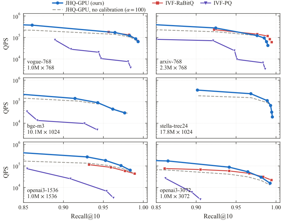
Fig. 3: Measured Recall@10–QPS frontiers, batch 1,024. Four datasets carry complete JHQ/IVF-RaBitQ curves; the two largest show the baselines that could be built and searched on the tested card. Sweep endpoints are measured endpoints, not architectural recall ceilings.
