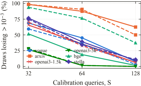
(a) Held-out quality risk
