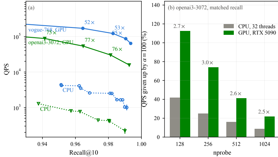
Fig. 4: GPU against CPU JHQ at the same index parameters. (a) Both sides’ ( \alpha , nprobe ) envelopes, annotated with the ratio at matched recall; open markers are the CPU points the envelope is taken over. (b) What the \alpha budget is worth on each processor, at matched recall on openai3-3072 — the reason the budget is worth choosing on a GPU and not on a CPU.
