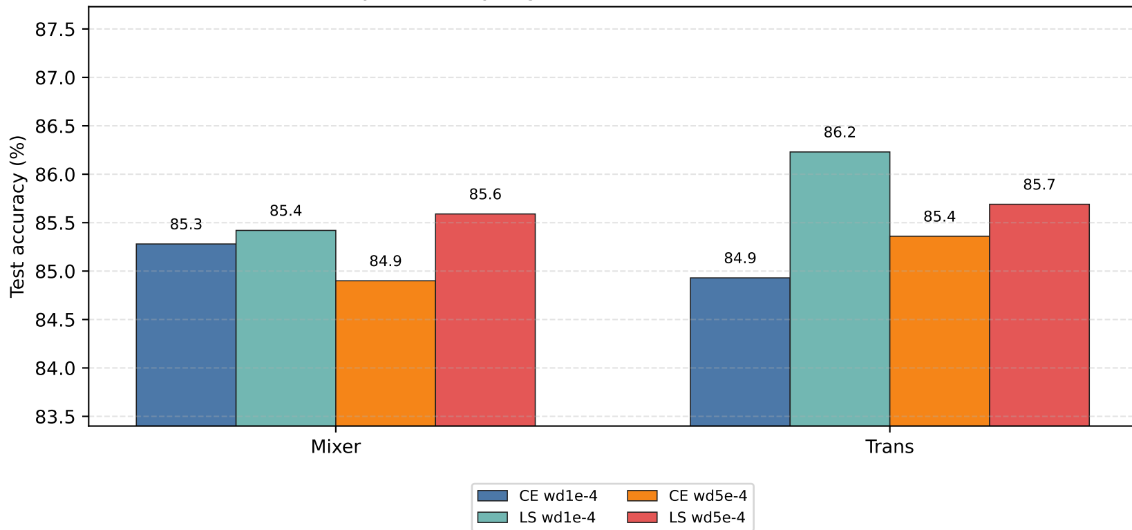
Hybrid-family regularization controls, seed 2020
