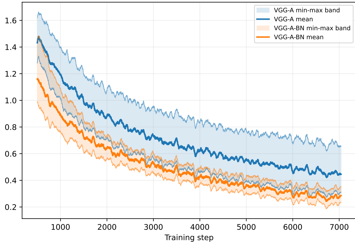
Zoom after first 500 steps
