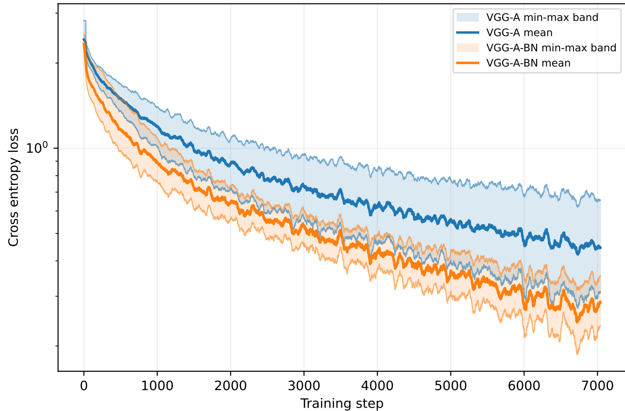
Full trajectory, log scale
