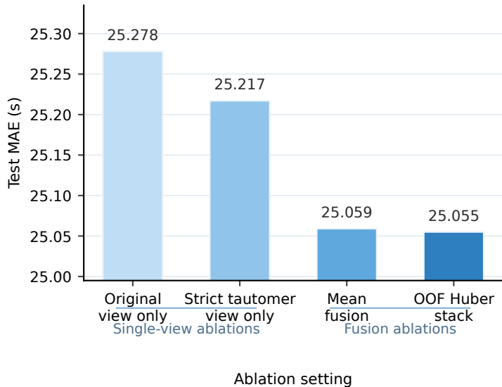
A Dual-view and fusion ablation
