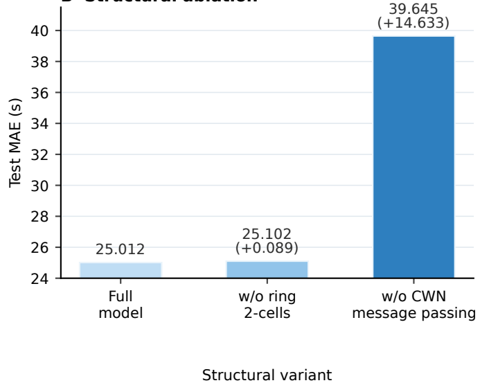
B Structural ablation
