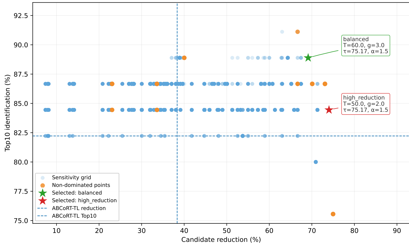
MetaboBase_evaluable45: sensitivity of RT-aware guarded soft reranking
