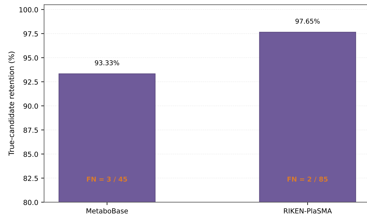
True-candidate retention and false negatives
