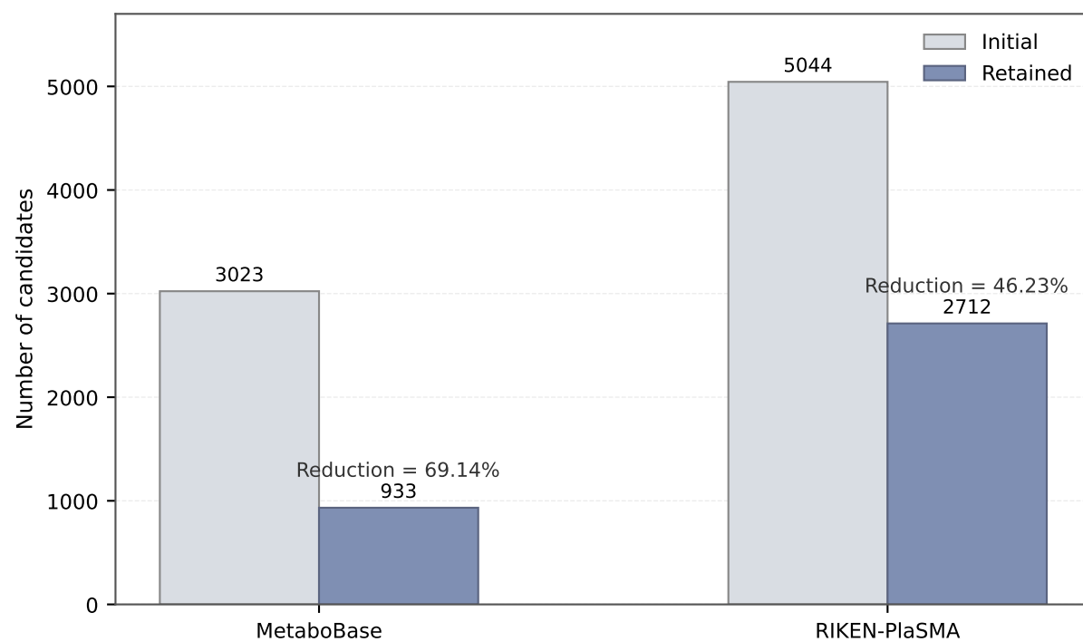
Candidate-space reduction by TC-TopoRT
