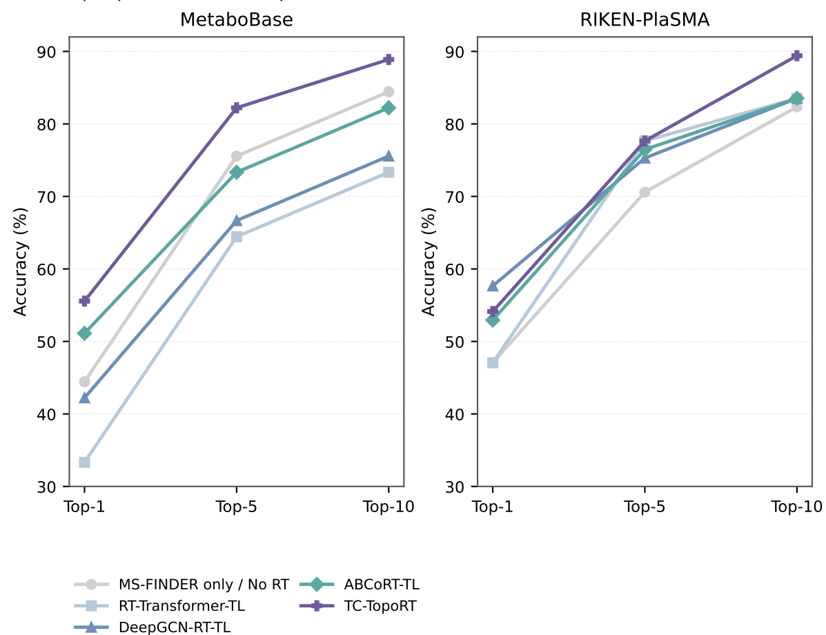
Top-k prioritization comparison
