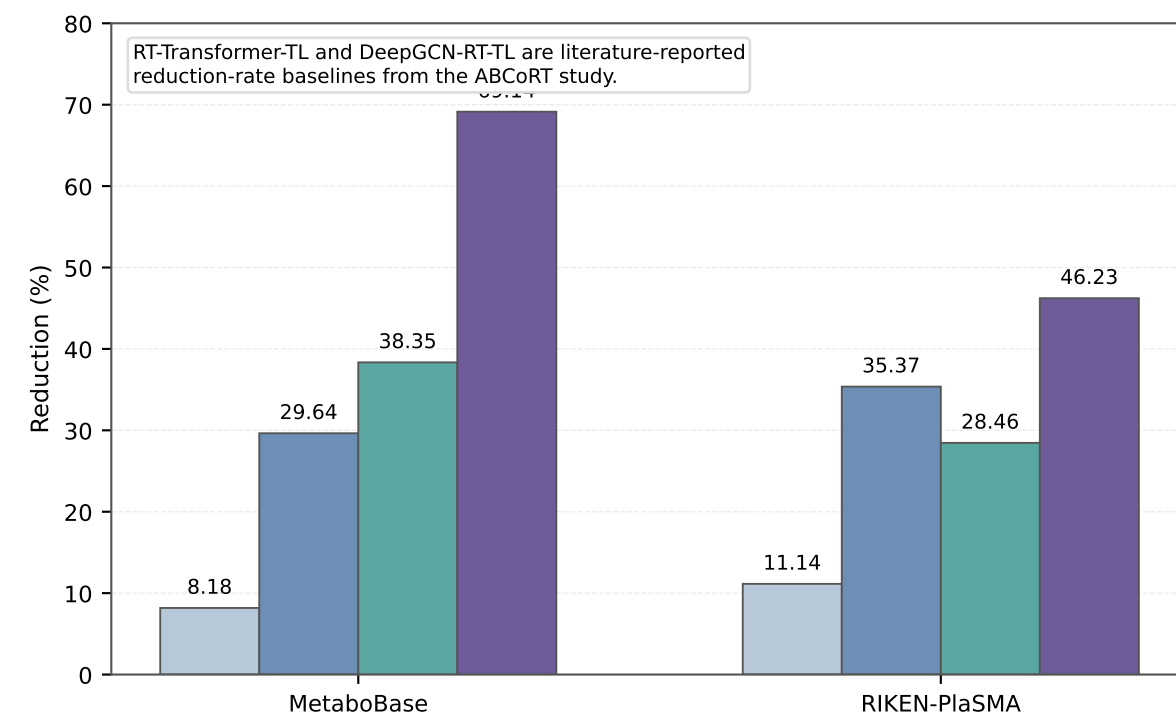
Candidate reduction compared with RT-filtering baselines
