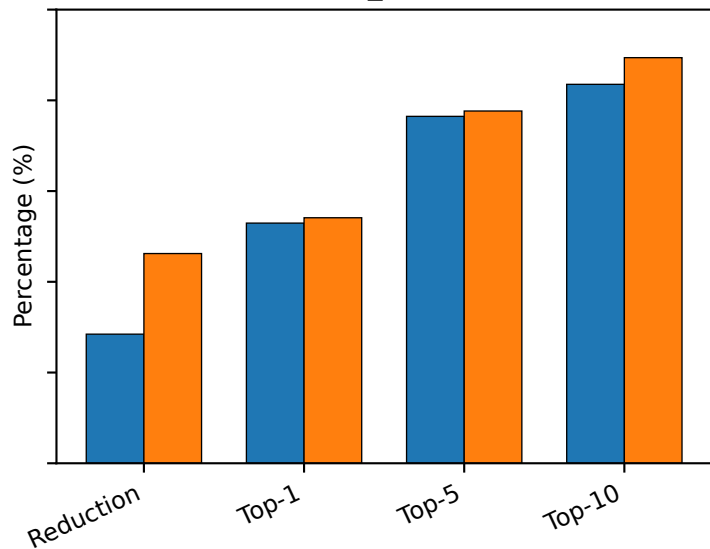
RIKEN_PlaSMA
