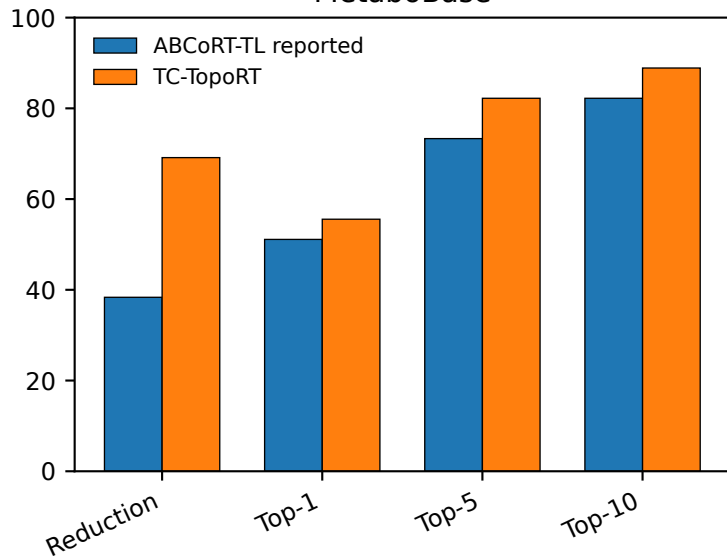
MetaboBase
