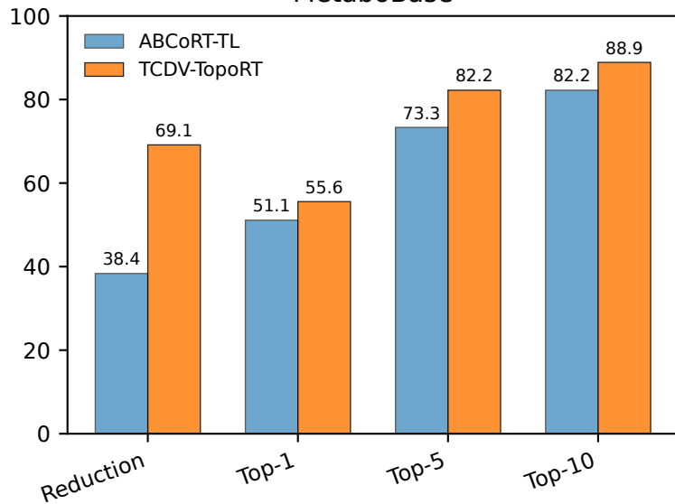
MetaboBase
