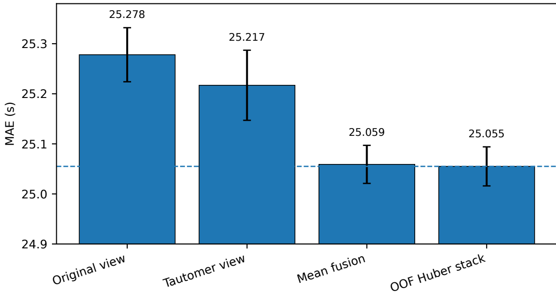
Dual-view and prediction-level fusion ablation
