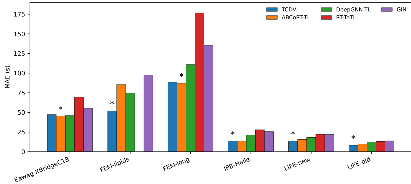
External transfer performance across chromatographic datasets
