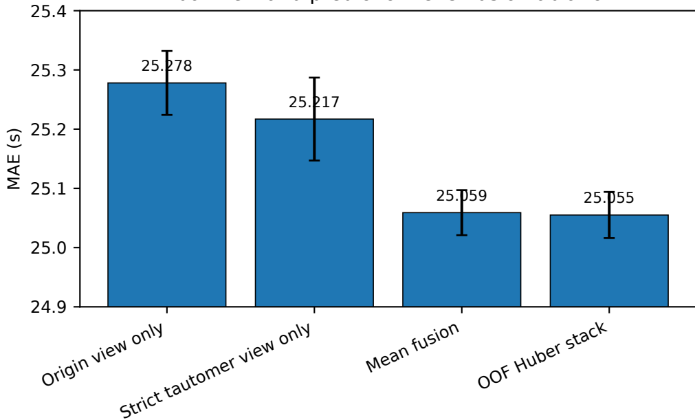
Dual-view and prediction-level fusion ablation
