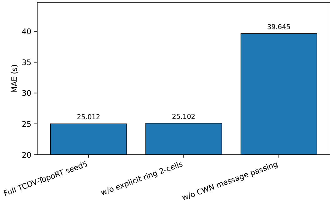
Topology-aware structural ablation
