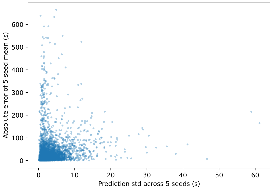
Seed disagreement vs prediction error
