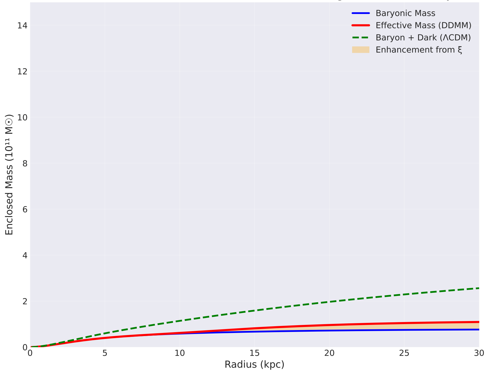
DDMM Achieves Same Effect as Dark Matter Through Enhanced Gravity
