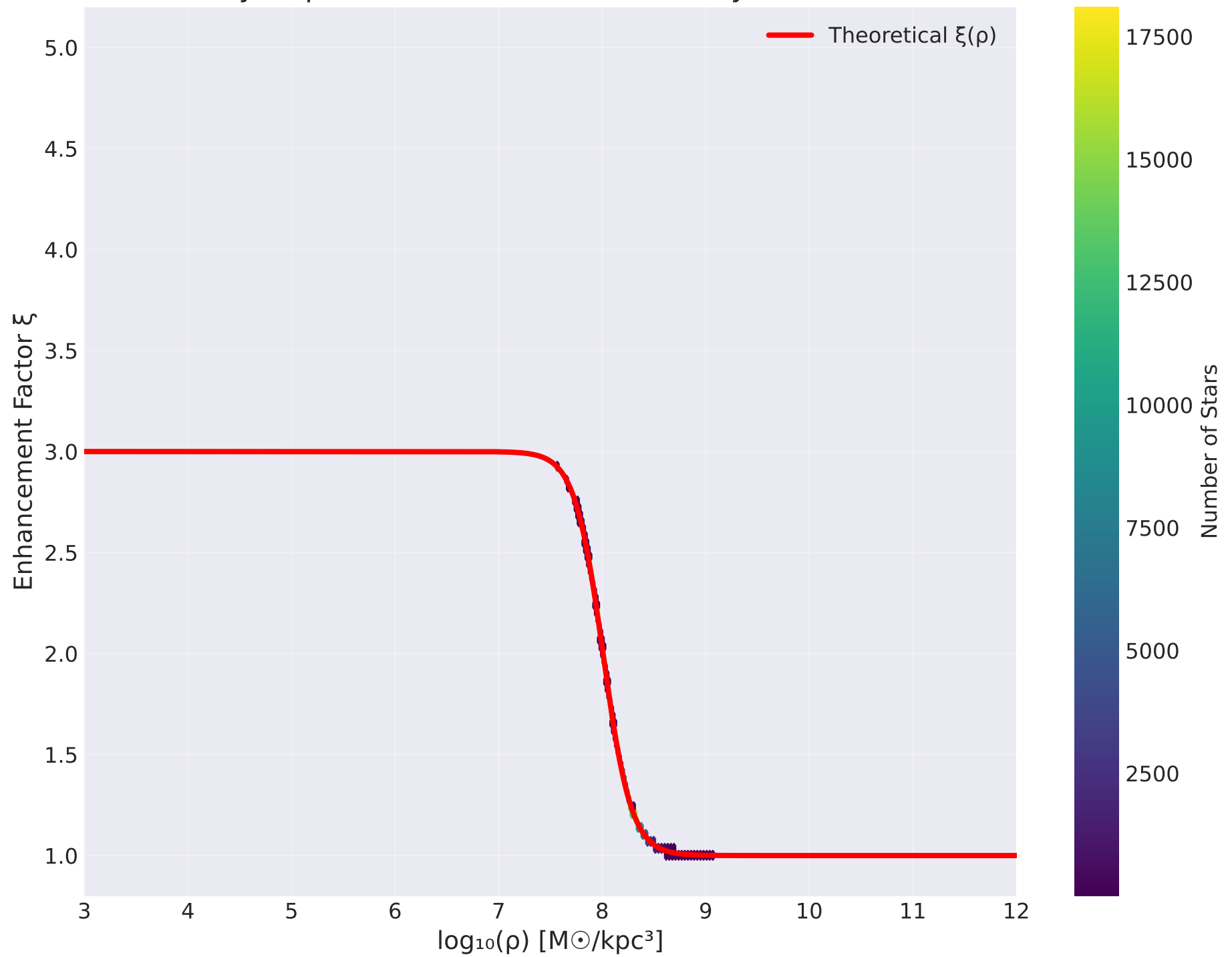
Density-Dependent Enhancement: Theory Matches Data
