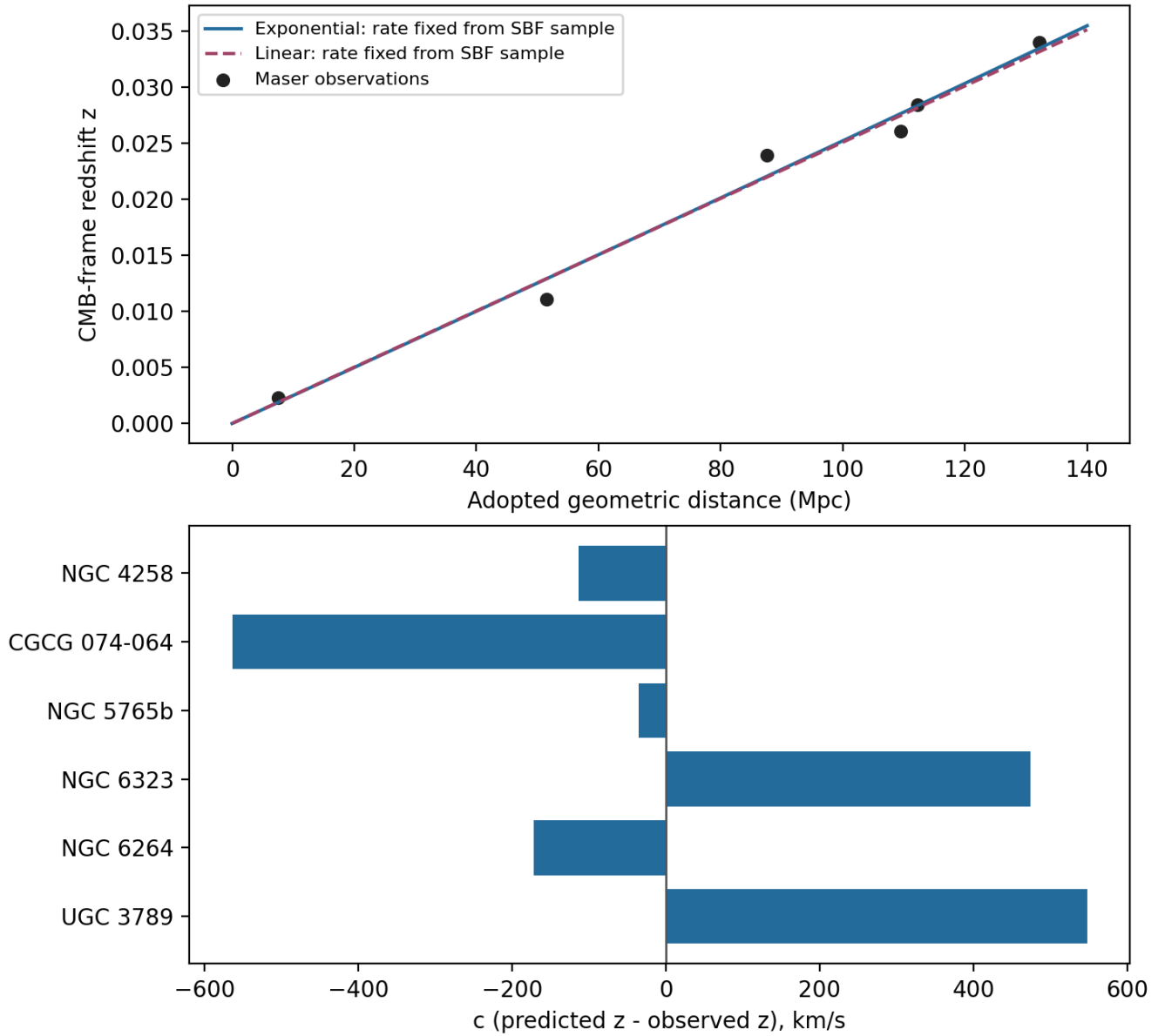
Figure 3. Six maser galaxies with the previously fixed rates. Neither curve is fitted to these six points. The lower panel retains every signed exponential residual; distances are held fixed and no uncertainty envelope is asserted.
