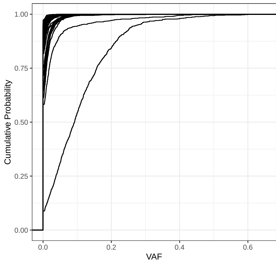
VAF ECDF ( KIA2 – Disease )
