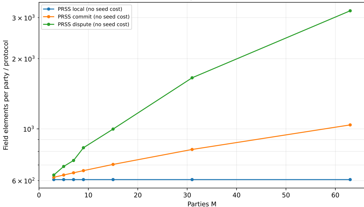
PRSS profile sensitivity: seed cost excluded (n=8)
