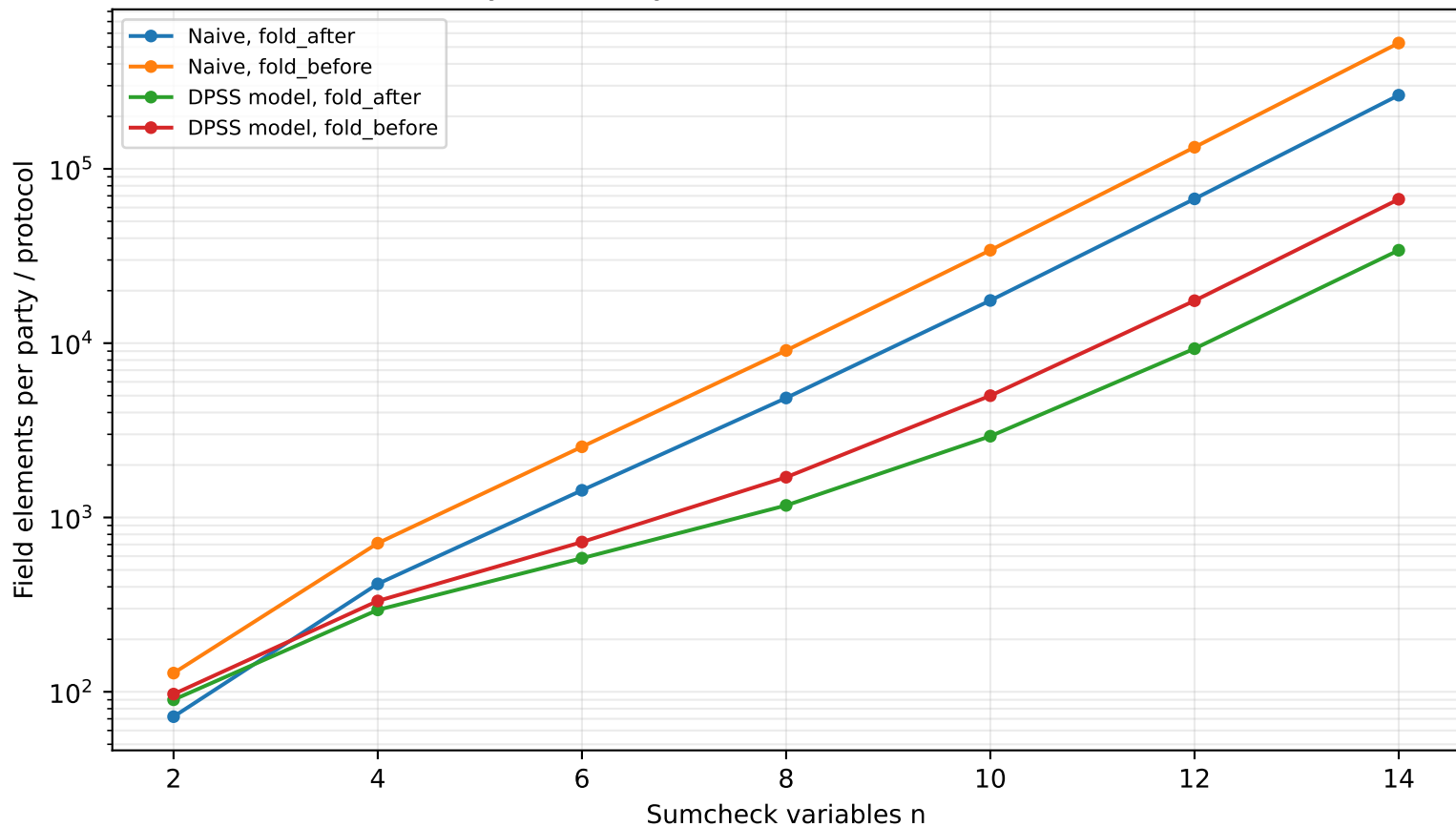
Boundary sensitivity: after 1..n-1 vs before 0..n-2 (M=9)
