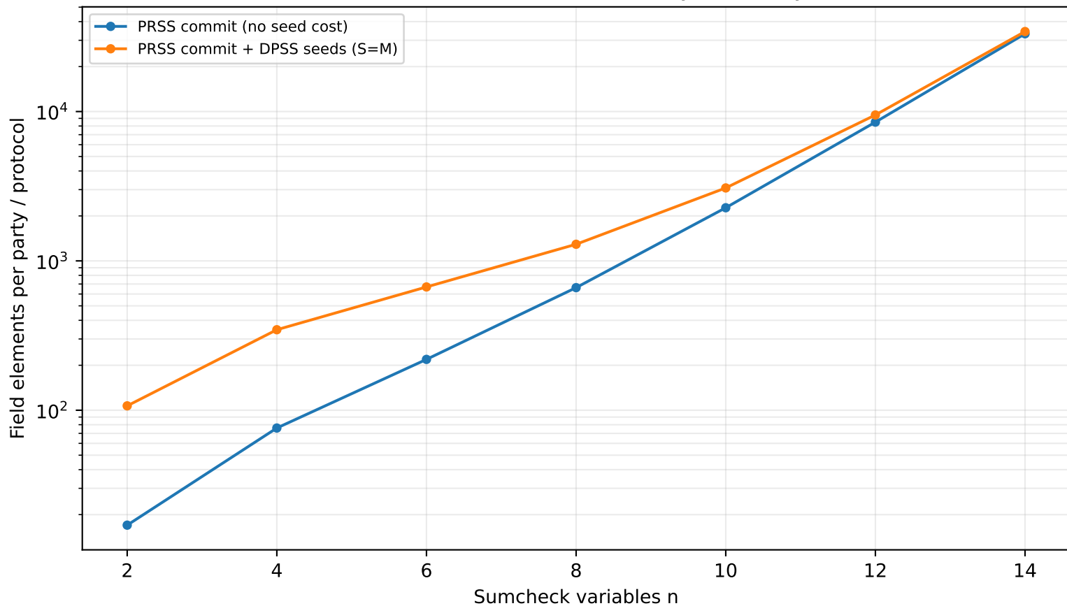
PRSS seed-refresh cost: S=M at every boundary ( M=9 )
