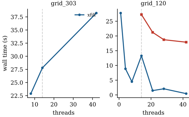
Fig. 2. Wall time vs. thread count, xfill vs. orca-solver, on two grids known to be hard for restart-based search (45s cap; orca-solver missing from a panel means every one of its 7 thread counts timed out; a third grid, grid_115, times out for both solvers at every thread count tested and is omitted, see text). grid_120 is the clearest case: xfill improves roughly 65\times from 1 to 42 threads while orca-solver stays flat and cannot solve at all below 14.
