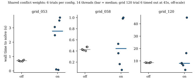
Fig. 5. Shared-conflict-weight ablation: 6 trials per configuration, 14 threads (bar = median; grid 120 trial 6 timed out at 45s, off-scale). Grey = mechanism off, blue = on (this paper’s default). Bars mark the median; the spread is the finding.
