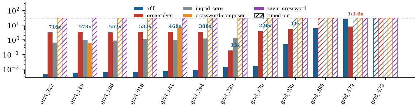
Wall time per grid, all five solvers, scraped 15x15 grids (geomean 108x)
