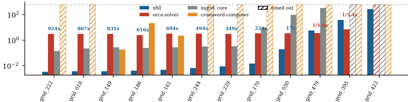
Wall time per grid, four solvers, scraped 15x15 grids (geomean 107x)
