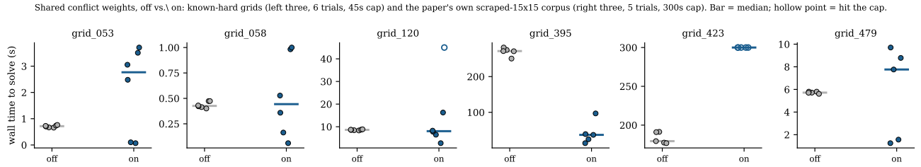
Fig. 1. Shared-conflict-weight ablation, off vs. on, 14 threads: a known-hard grid list also used in Fig. 2 (left three, 6 trials, 45s cap) and three grids from the paper’s own scraped- 15 \times 15 corpus (right three, 5 trials, 300s cap; the other 9 of 12 solve in under a second and are omitted). Bars mark the median; hollow points hit the cap. Shared weights are not uniformly better: the same win/wash/loss pattern appears independently on both grid sets.
