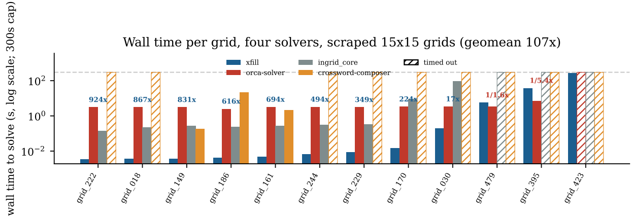
Fig. 3. Wall time to solve (log scale, 300s cap), four solvers, per scraped 15 \times 15 grid, sorted by xfill’s time. Hatched bars mark a timeout; crossword-composer times out on most grids, the same pattern reported by count in Section V-D (savin_crossword is excluded entirely, also Section V-D). Label above the xfill/orca-solver pair is orca-solver time / xfill time; two grids (grid_395, grid_479) favor orca-solver, and on grid_423 orca-solver cannot solve it at all at this cap while xfill does, in 270s.
