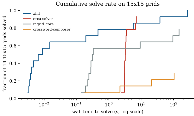
Fig. 4. Cumulative fraction of real 15 \times 15 grids solved by wall time (log scale), 300s cap. The point is the horizontal gap between curves, not the final height: xfill’s curve is shifted roughly two orders of magnitude left of ingrid_core’s and orca-solver’s, meaning it reaches the same solved fraction far sooner across the entire distribution – and it is also the only curve that reaches 1.0, solving all 14.
