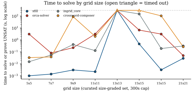
Fig. 2. Time to solve or prove UNSAT by grid size, curated set, 300s cap (log scale; open triangle = timed out). A solved/not-solved view of this same data would show xfill , orca-solver , and ingrid_core essentially tied, since all three succeed on the same grids here – the actual difference is that xfill ’s line sits one to three orders of magnitude below the others at every size except 13 \times 13 (every solver times out together) and 21 \times 21 (an easy UNSAT proof every solver resolves in well under a second regardless).
