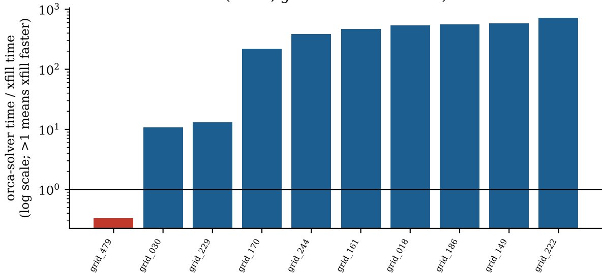
Per-grid speedup, xfill vs. orca-solver, scraped 15x15 grids, where both solved (n=10, geometric mean 108x)
