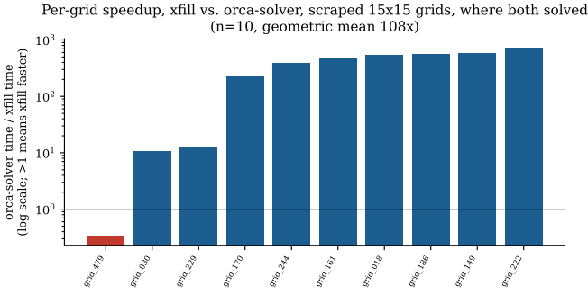
Fig. 3. Per-grid speedup (orca-solver time / xfill time, log scale) on the scraped 15 \times 15 grids both solvers solved. Bars above the line mean xfill is faster; only one of 10 falls below it.
