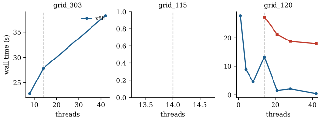
Fig. 2. Wall time vs. thread count, xfill vs. orca-solver, on three grids known to be hard for restart-based search (45s cap; orca-solver missing from a panel means every one of its 7 thread counts timed out). grid_120 is the clearest case: xfill improves roughly 65 \times from 1 to 42 threads while orca-solver stays flat and cannot solve at all below 14.
