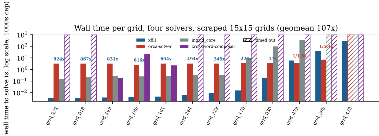
Fig. 4. Wall time to solve (log scale, 1000s cap), four solvers, per scraped 15 \times 15 grid, sorted by xfill’s time. Hatched bars mark a timeout; crossword-composer times out on most grids, the same pattern reported by count in Section V-E. Label above the xfill/orca-solver pair is orca-solver time / xfill time; two grids (grid_395, grid_479) favor orca-solver, and on grid_423 orca-solver cannot solve it even at this cap while xfill does, in 270s.
