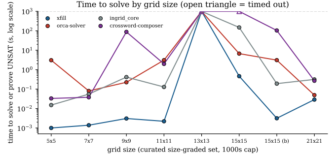
Fig. 3. Time to solve or prove UNSAT by grid size, curated set, 1000s cap (log scale; open triangle = timed out; a second, denser 15 \times 15 grid is marked (b)). A solved/not-solved view of this same data would show xfill, orca-solver, and ingrid_core essentially tied, since all three succeed on the same grids here: the actual difference is that xfill’s line sits one to nearly five orders of magnitude below the others at every size except 13 \times 13 (every solver times out together) and 21 \times 21 (an easy UNSAT proof every solver resolves in well under a second regardless).
