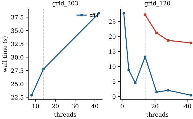
Fig. 2. Wall time vs. thread count, xfill vs. orca-solver, on two grids known to be hard for restart-based search (45s cap; dashed line = 14 physical cores; orca-solver missing from a panel means all 7 of its thread counts timed out; a third grid, grid_115, times out for both solvers at every thread count tested and is omitted, see text). grid_120 is the clearest case: xfill improves roughly 65\times from 1 to 42 threads while orca-solver stays flat and cannot solve at all below 14.
