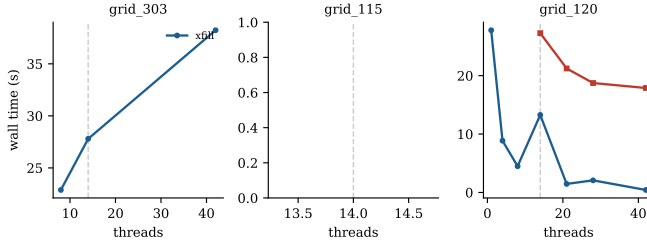
Fig. 1. Wall time vs. thread count, xfill vs. orca-solver, on three grids known to be hard for restart-based search (45s cap; orca-solver missing from a panel means every one of its 7 thread counts timed out). grid_120 is the clearest case: xfill improves roughly 65\times from 1 to 42 threads while orca-solver stays flat and cannot solve at all below 14.
