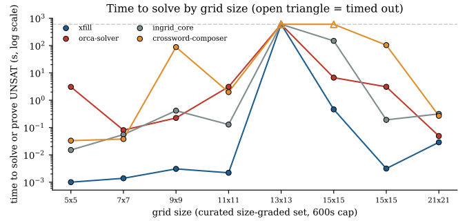
Fig. 2. Time to solve or prove UNSAT by grid size, curated set, 600s cap (log scale; open triangle = timed out). A solved/not-solved view of this same data would show xfill, orca-solver, and ingrid_core essentially tied, since all three succeed on the same grids here – the actual difference is that xfill’s line sits one to three orders of magnitude below the others at every size except 13 \times 13 (every solver times out together) and 21 \times 21 (an easy UNSAT proof every solver resolves in well under a second regardless).
