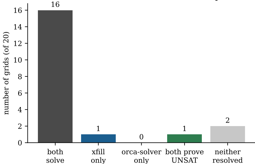
xfill vs. orca-solver: outcome overlap
