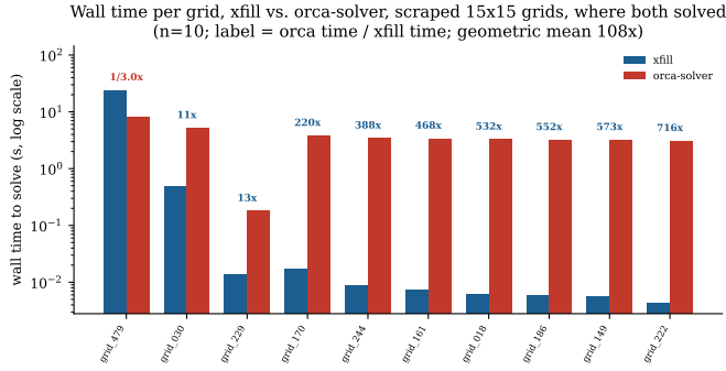
Fig. 3. Wall time to solve (log scale), xfill vs. orca-solver, per scraped 15 \times 15 grid both solved. Label is orca-solver time / xfill time; only grid_479 favors orca-solver.
