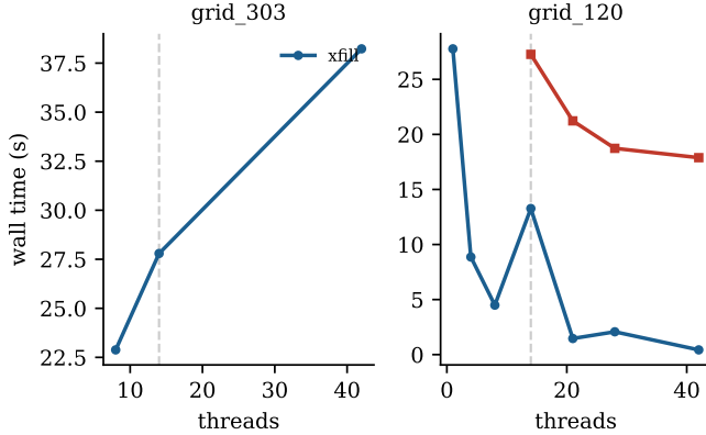
Fig. 2. Wall time vs. thread count, xfill vs. orca-solver, on two grids known to be hard for restart-based search (45s cap; dashed line = 14 physical cores; orca-solver missing from a panel means every one of its 7 thread counts timed out; a third grid, grid_115, times out for both solvers at every thread count tested and is omitted, see text). grid_120 is the clearest case: xfill improves roughly 65\times from 1 to 42 threads while orca-solver stays flat and cannot solve at all below 14.
