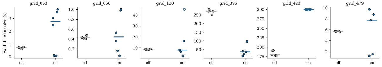
Fig. 1. Shared-conflict-weight ablation, off vs. on, 14 threads: a known-hard grid list also used in Fig. 2 (left three, 6 trials, 45s cap) and three grids from the paper’s own scraped- 15 \times 15 corpus (right three, 5 trials, 300s cap; the other 9 of 12 solve in under a second and are omitted). Bars mark the median; hollow points hit the cap. Shared weights are not uniformly better: the same win/wash/loss pattern appears independently on both grid sets.
