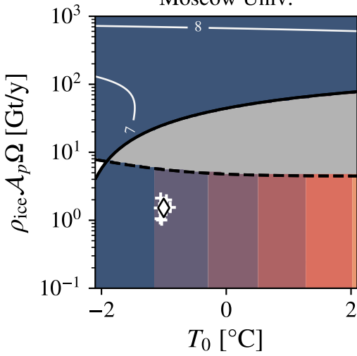
Moscow Univ.
