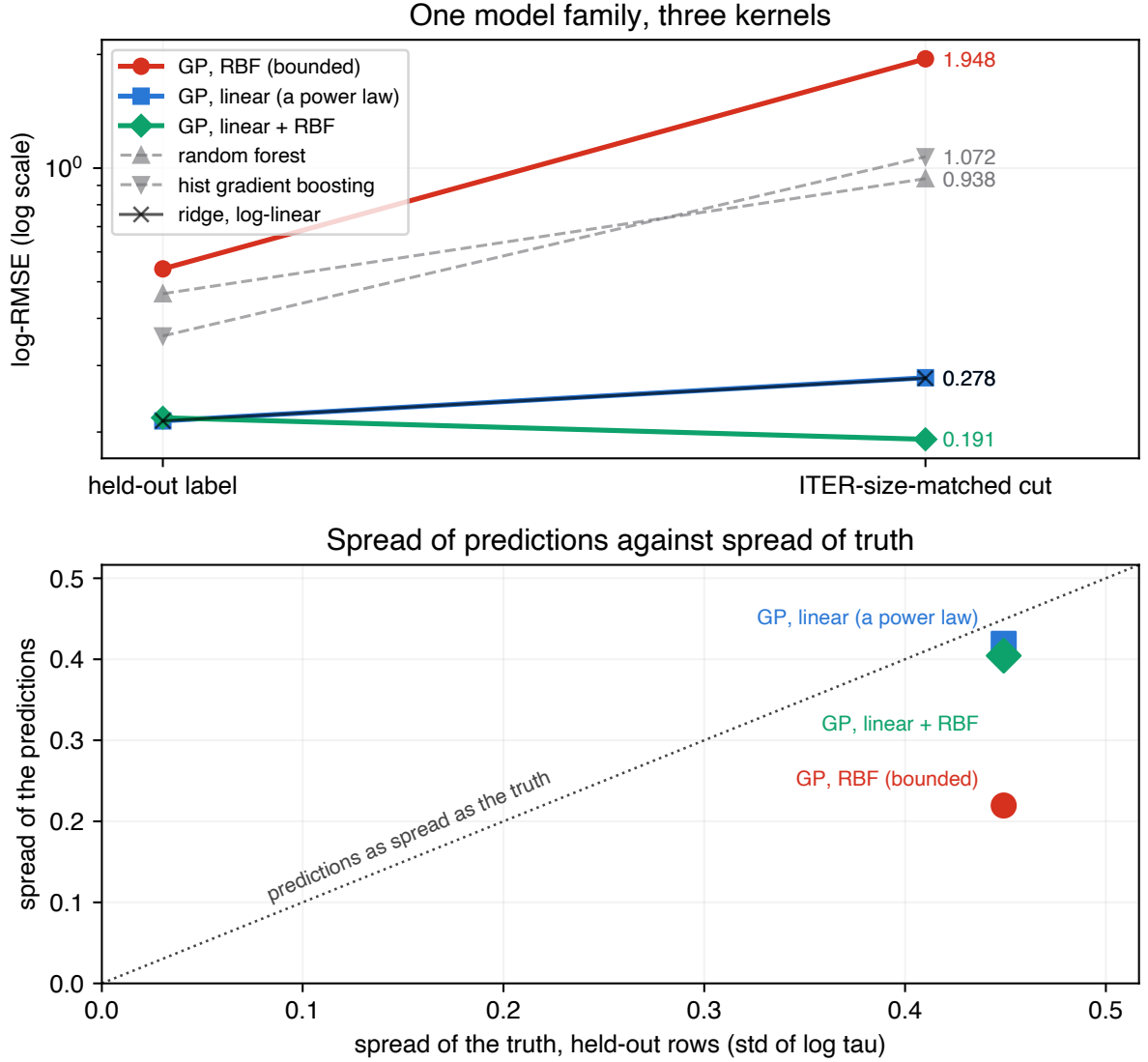
Figure S3: One model family, three kernels. Gaussian processes with a radial-basis-function (RBF) kernel, a linear (dot-product) kernel, and their sum. Top: log-RMSE on a held-out label and at the ITER-size-matched cut. The kernels differ in whether they permit a trend that continues at long range; adding the linear component also enlarges the function class. Bottom: spread of the predictions against spread of the truth on the held-out rows. A model whose posterior has reverted to its prior mean predicts nearly the same value everywhere, so its spread sits near zero however good its in-range fit was: the same failure a tree ensemble shows when it cannot exceed its largest training target, reached by a different route.
