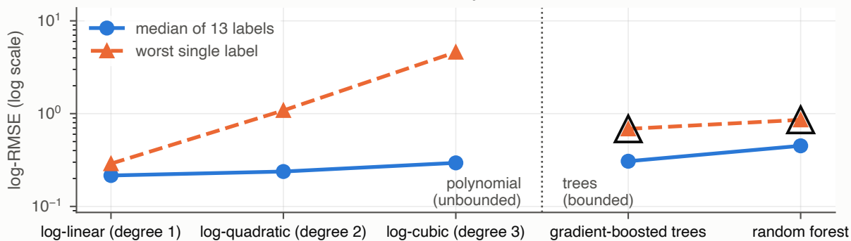
The flexibility ladder
