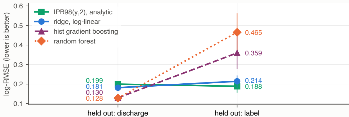
Interpolation against extrapolation
