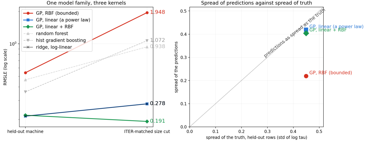
Figure 6: One model family, three kernels. Left: RMSLE on a held-out machine and at the ITER-matched cut. The kernels differ in whether they permit a trend that continues at long range; adding the linear component also enlarges the function class. Right: spread of the predictions against spread of the truth on the held-out rows. A model that has reverted to its prior mean sits near zero however good its in-range fit was, which is the tree ceiling of Sec. 5.1 reached by a different route.
