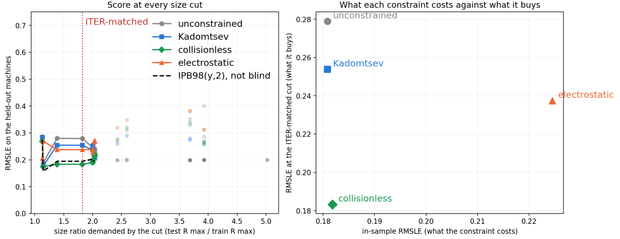
Figure 3: Cost against benefit across the size sweep. Left: the score at every size cut for the constrained and unconstrained fits, with underpowered cuts drawn faint and excluded from claims. Right: what each constraint costs in sample against what it buys at the ITER-matched cut. The constraint costs almost nothing where the data is plentiful and pays where it is not, and more physics is not monotonically better: the hierarchy has an optimum in its middle, at the collisionless rung.
