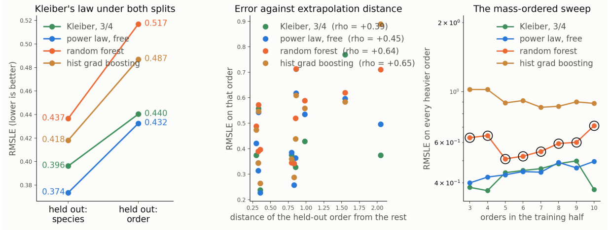
Figure 4: Kleiber’s law under the same three splits. Left: no inversion, because the trees lose under both splits and so have no interpolation margin to give up. Middle: error against extrapolation distance, rising for the flexible models as it does on HDB5. Right: the mass-ordered sweep, with the circled points marking cuts where the random forest is held inside its training range.
