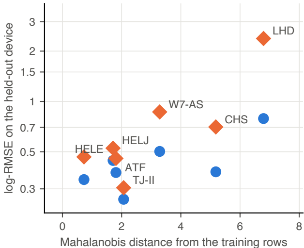
Holdout error against distance
