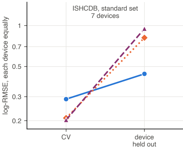
Known devices against an unseen one
