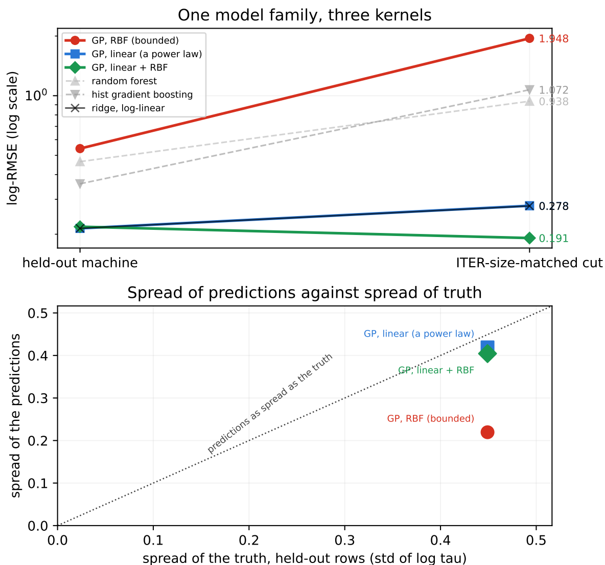
Figure 4: One model family, three kernels. Top: log-RMSE on a held-out machine and at the ITER-size-matched cut. The kernels differ in whether they permit a trend that continues at long range; adding the linear component also enlarges the function class. Bottom: spread of the predictions against spread of the truth on the held-out rows. A model that has reverted to its prior mean sits near zero however good its in-range fit was, which is the tree ceiling of Sec. 5.1 reached by a different route.
