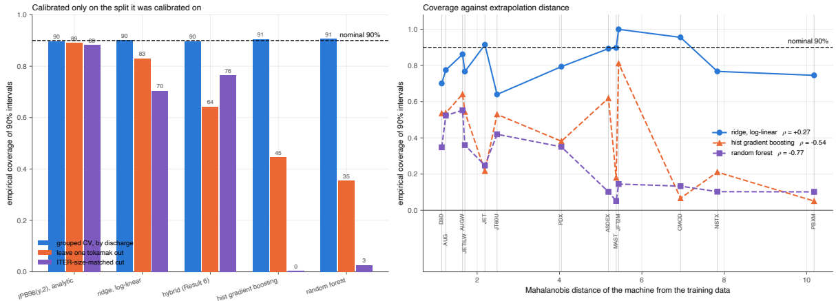
Figure 2: The interval collapse. Left: empirical coverage of nominal 90% split-conformal intervals for each model under the three splits, against the nominal line. Every model is calibrated under grouped cross-validation, and only the linear and constrained fits stay near it once the held-out unit becomes a whole label and then a size range. Right: per-label coverage against the Mahalanobis distance of the label from the training data. Under grouped cross-validation coverage is flat on the nominal line at every distance; under leave-one-label-out the tree ensembles fall away with distance and the power law does not. Interval widths behind both panels move by under 1.5% between the splits, so what is drawn is intervals that keep their size and lose their coverage.
