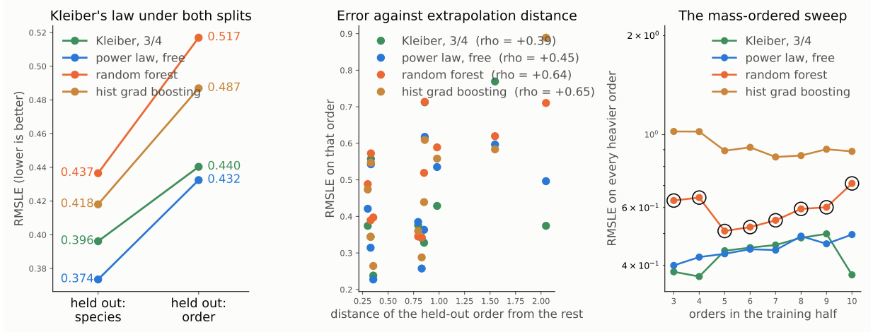
Figure 5: Kleiber’s law under the same three splits. Left: no inversion, because the trees lose under both splits and so have no interpolation margin to give up. Middle: error against extrapolation distance, rising for the flexible models as it does on HDB5. Right: the mass-ordered sweep, with the circled points marking cuts where the random forest is held inside its training range.
