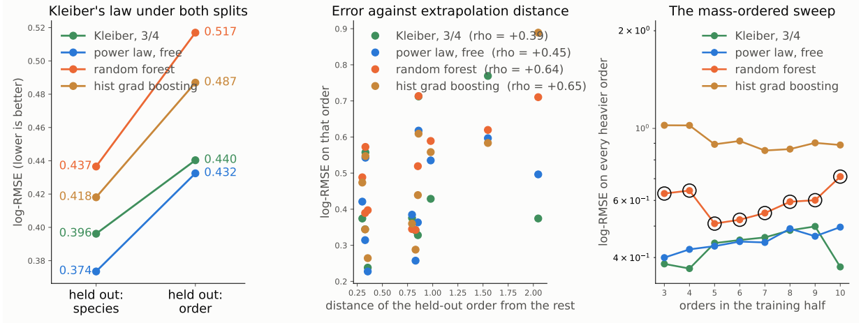
Figure 5: Kleiber’s law under the same three splits. Left: no inversion, because the trees lose under both splits and so have no interpolation margin to give up. Middle: error against extrapolation distance, rising for the flexible models as it does on HDB5. Right: the mass-ordered sweep, with the circled points marking cuts where the random forest is held inside its training range.
