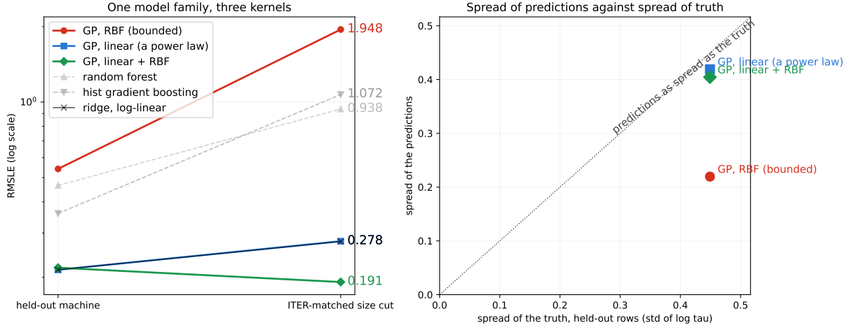
Figure 4: One model family, three kernels. Left: log-RMSE on a held-out machine and at the ITER-size-matched cut. The kernels differ in whether they permit a trend that continues at long range; adding the linear component also enlarges the function class. Right: spread of the predictions against spread of the truth on the held-out rows. A model that has reverted to its prior mean sits near zero however good its in-range fit was, which is the tree ceiling of Sec. 5.1 reached by a different route.
