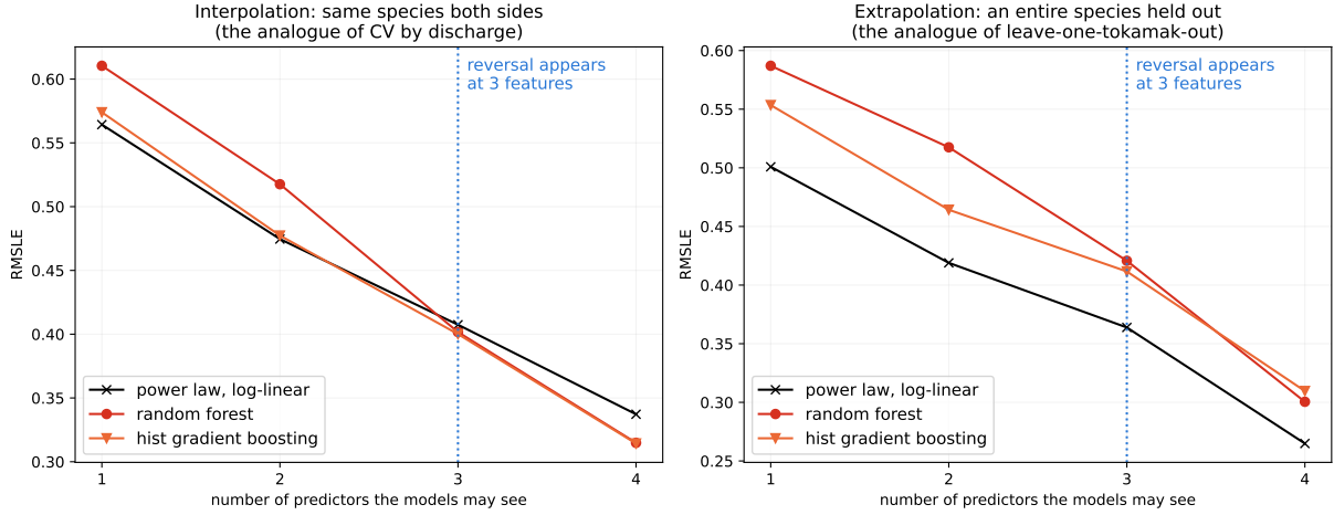
Figure 6: The reversal’s precondition, on 3599 plants held fixed. Left: the interpolation split, where every species appears on both sides. Right: an entire species held out. Only the number of predictors varies. The left curves cross; the right ones do not.
